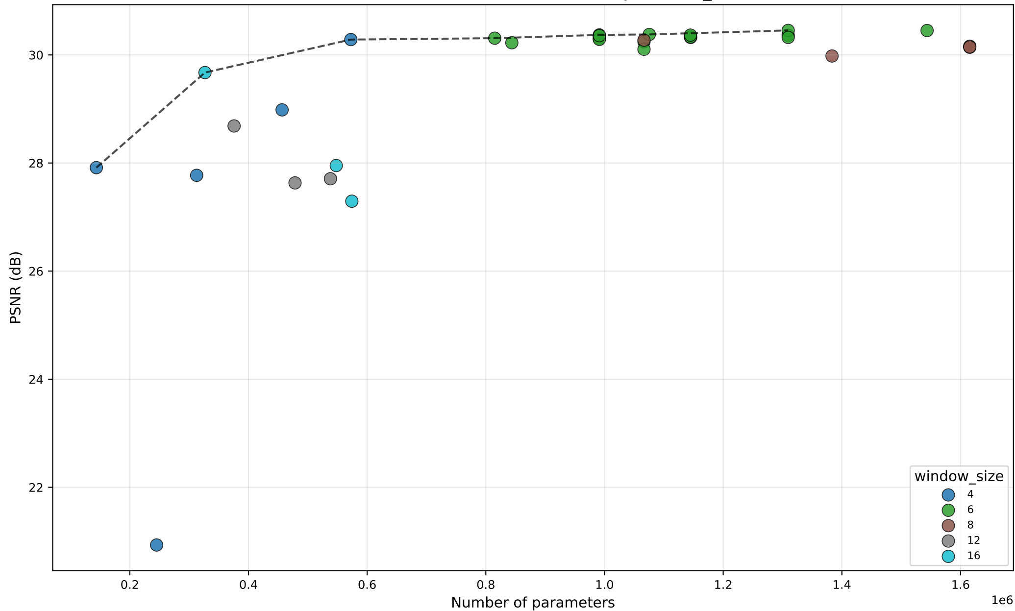
PSNR vs #Params — SRFormer — by window_size
